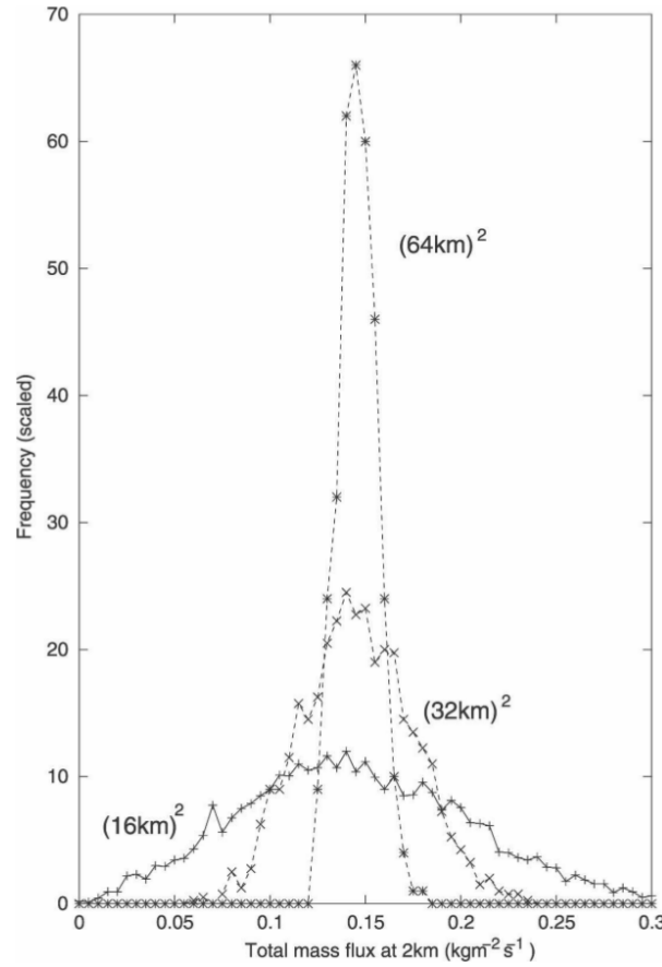
Figure 2.5: From Plant and Craig (2008), their Fig. 1. Shows the frequency distribution of total convective mass flux per unit area at a height of 2 km from the CRM simulation of Cohen and Craig (2006). The vertical axis is scaled so that all averaging areas can be plotted on the same axis.
