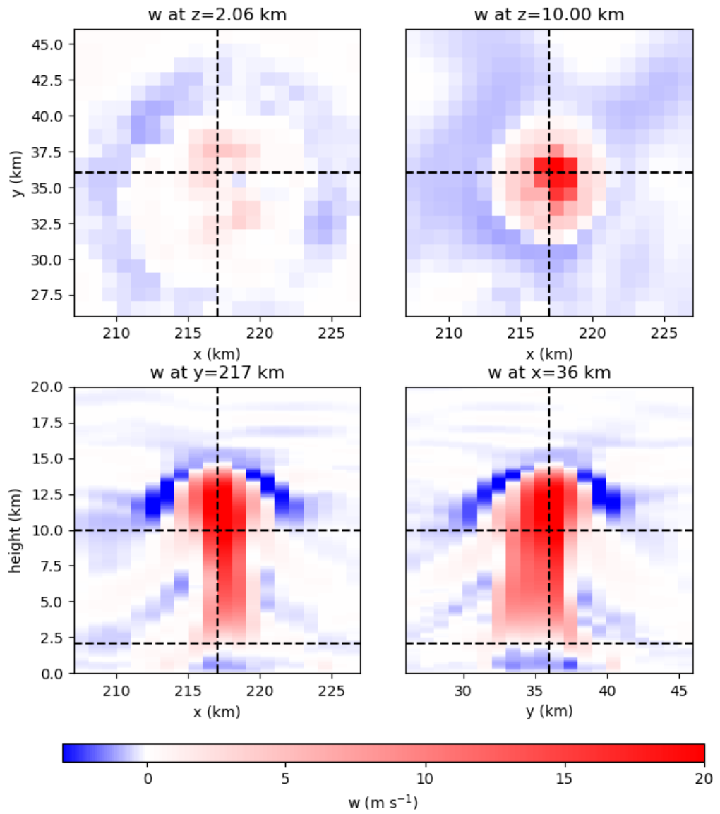
Figure 4.11: Horizontal and vertical cross-sections of w for S0W0F. The two top panels show horizontal cross-sections at 2.06 km (left) and 10 km (right). The bottom panels show a x-z cross-section (left) and y-z cross section (right). In each panel, the positions of the other cross-sections are shown by a black dashed line.
