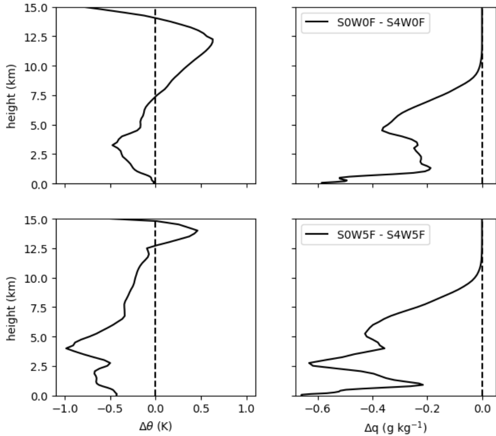
Figure 4.18: Difference between no-shear and shear experiments for \theta (potential temperature – left) and q (specific humidity – right), where the difference is the no-shear experiment minus the shear experiment. Top shows the W0 experiments, and bottom shows the W5 experiments.
