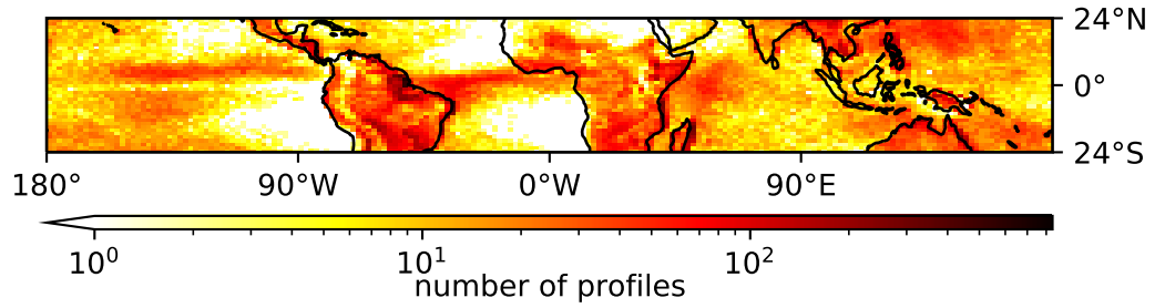
Figure 3.2: Heatmap of grid-columns that have been filtered based on CAPE and maximum shear. The heatmap shows the number of profiles in each grid-column that have been kept after applying both filters to the output of the five years of the simulation. The data used is the 6-hourly climate model output described in Sect. 3.2.1.
