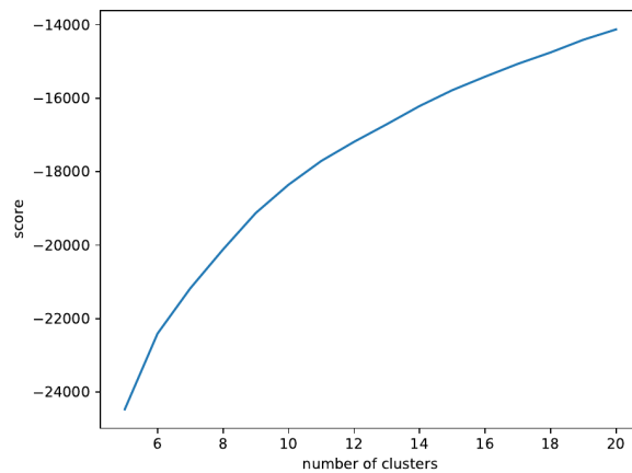
Figure A.1: K-means scores produced with different numbers of clusters. The score is a measure of the within-cluster variance, with a lower score indicating a higher variance. The score improves as more clusters are used. Such a diagram is commonly called an ‘elbow plot’. In this case no clear elbow, or kink in the curve, is seen. We therefore choose 10 clusters as a pragmatic choice to use to generate the RWPs.
